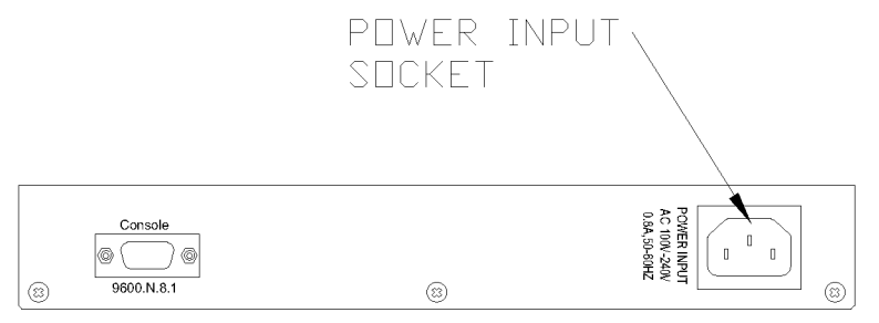
REAR VIEW
