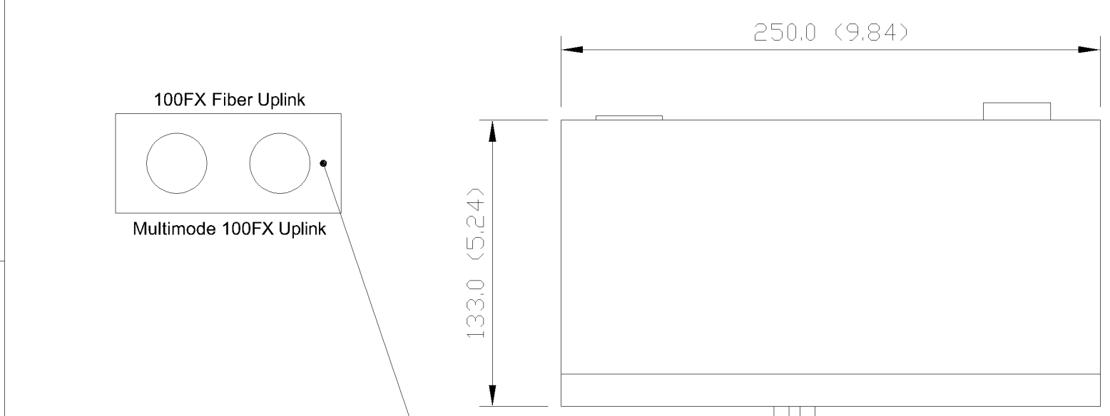
TOP VIEW
