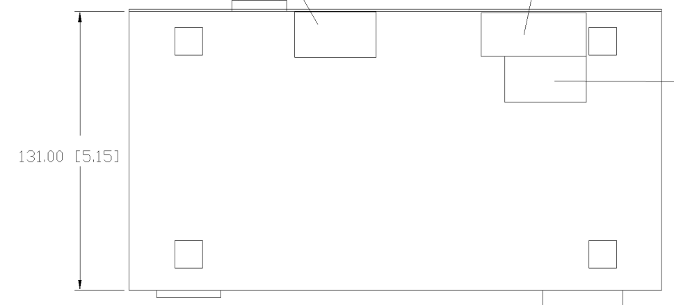
BASE VIEW DETAIL
